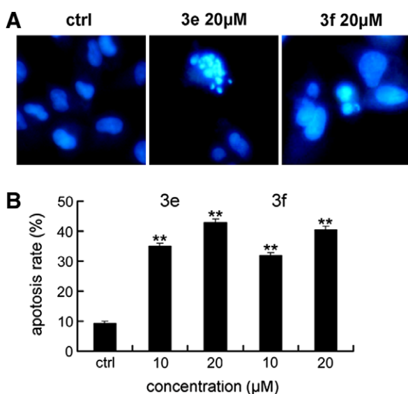
Figure 3. The compounds 3e and 3f induced apoptosis in A549 cells at 48 h ( p < 0.01 vs control, n = 3 ). Microscopic photographs (200×) were taken under a fluorescent microscope (Nikon).
