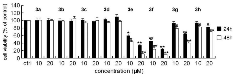
Figure 1. Effects of the compounds 3a–h on cell viability at 24 h (black bar) and 48 h (white bar).
