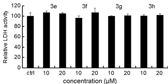
Figure 5. The compounds 3e–h did not induce necrosis in the cells at 48 h ( p > 0.05 vs control, n = 4 ).
