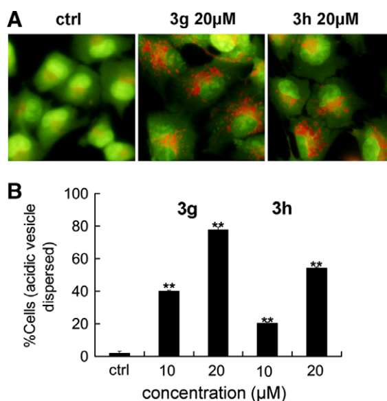
Figure 4. The compounds 3g and 3h increased the acidic vesicle level in the cells at 24 h ( p < 0.01 vs control, n = 3 ). Microscopic photographs (200×) were taken under a fluorescent microscope (Nikon).
