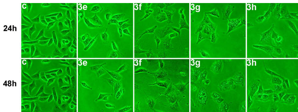
Figure 2. Morphological changes induced by compounds 3e–h at 20 μM. Microscopic photographs (200×) were taken under an inverted phase contrast microscope (Nikon).
